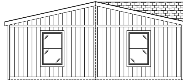
REAR ENDWALL
